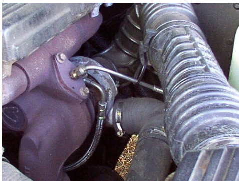
Thermocouple installed in exhaust manifold of a Land Rover 300Tdi engine
